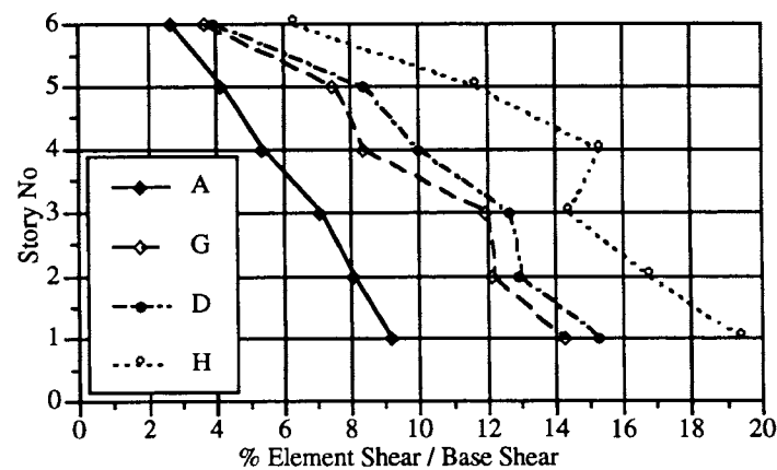
Fig. 11 Shear Ratio of Edge and Centre Elements-Group II
