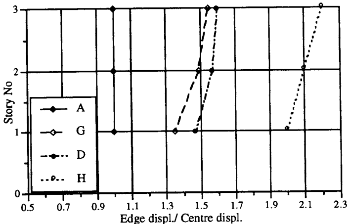
Fig. 9 Displacement Ratio of Edge and Centre Nodes-Group II
