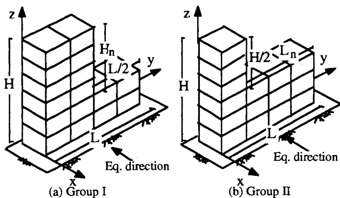
Fig. 7 Setback Configurations Considered in the Analysis
