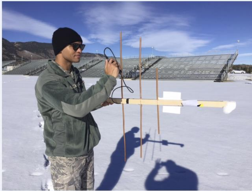
Figure 2. Transmitter Hunt with Directional Antenna in Two-Meter Band [1].
