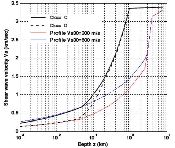
Fig. 5. Comparison of the results (shear wave velocity profile Vs. depth) of the Margaris and Klimis (1999) study and current paper for Greece (40N 22E)
