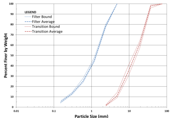
Fig. 1. Gradations of filter and transition materials in the stockpiles
