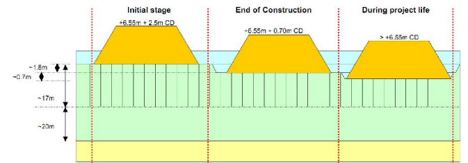
Fig. 14. PVD installation Alternative -2; PVDs installed up to partial depth i.e. 17m.
