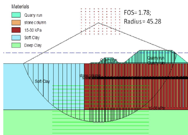
Fig.6 Calculated factor of safety for first stage breakwater construction (Bishop method)
