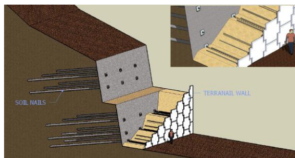
Fig. 1. Soil nailing linked to reinforced earth
