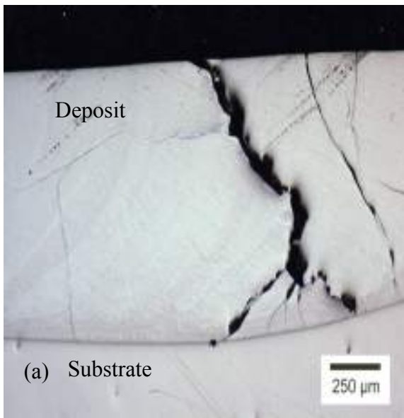
Fig. 4: Macrostructure of powder-2 deposit at 1000 W on (a) Ti6Al4V (shows macro-cracks); (b) SS316L (no macro-cracks) substrate.
