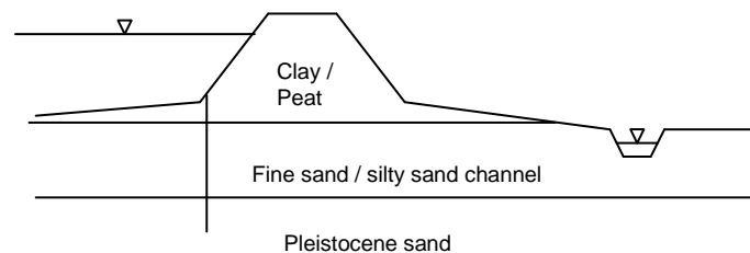
Figure 8: Scenario 1 - Dike cross section with large channel
