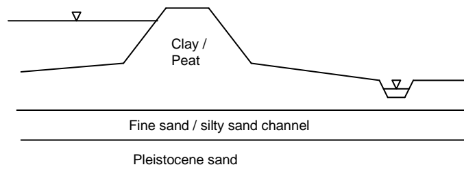
Figure 9: Scenario 2 - Dike cross section with small channel
