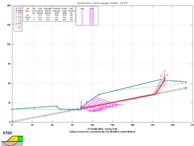
Fig. 3 Slope stability 2D analysis results
