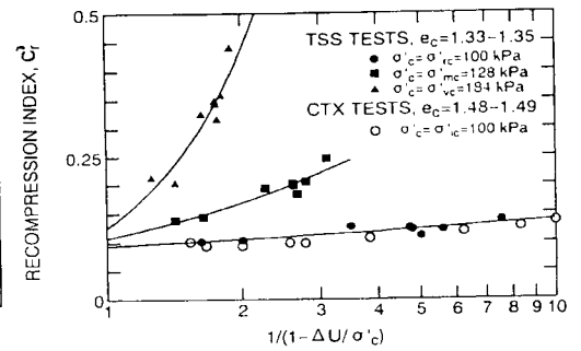
Fig.11 Comparison of recompression indices
