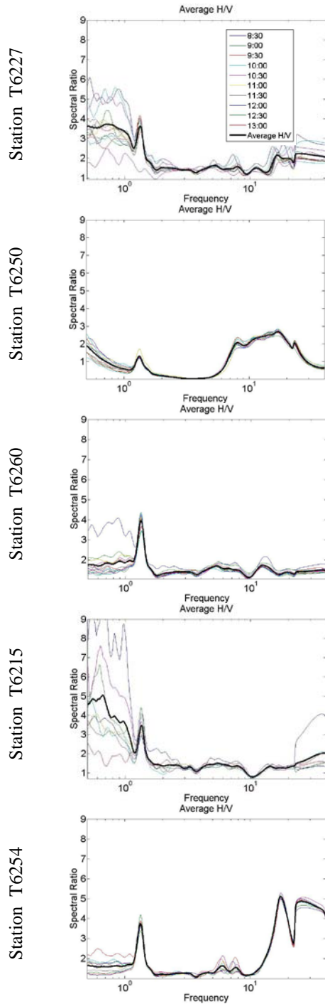
Fig. 2. The H/V curves for stations along the longitudinal profile.
