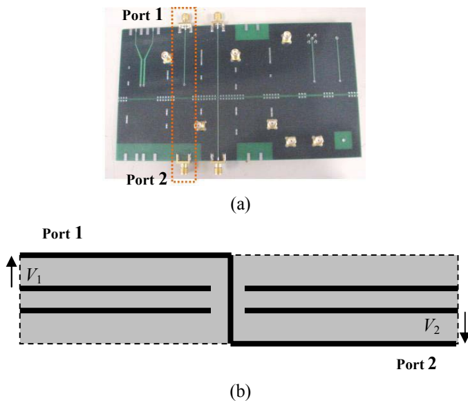
Figure 3. Test board: (a) general view and (b) its stack-up.
