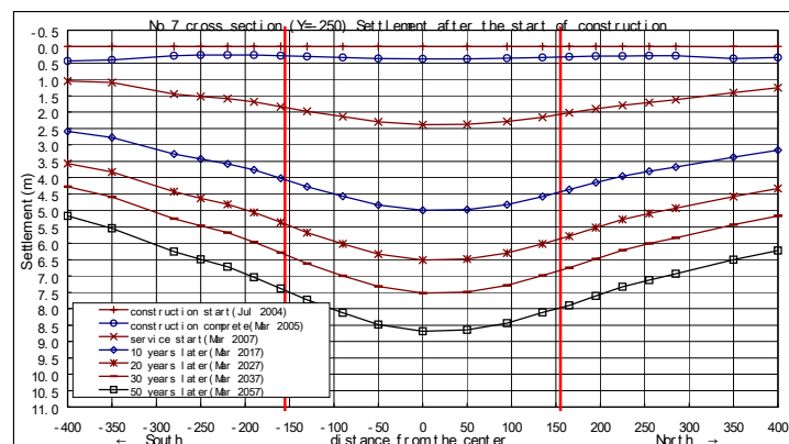
Fig. 17. Settlement Predictions in Cross sections
