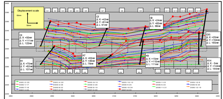
Fig. 31. Horizontal displacement of Underpass
