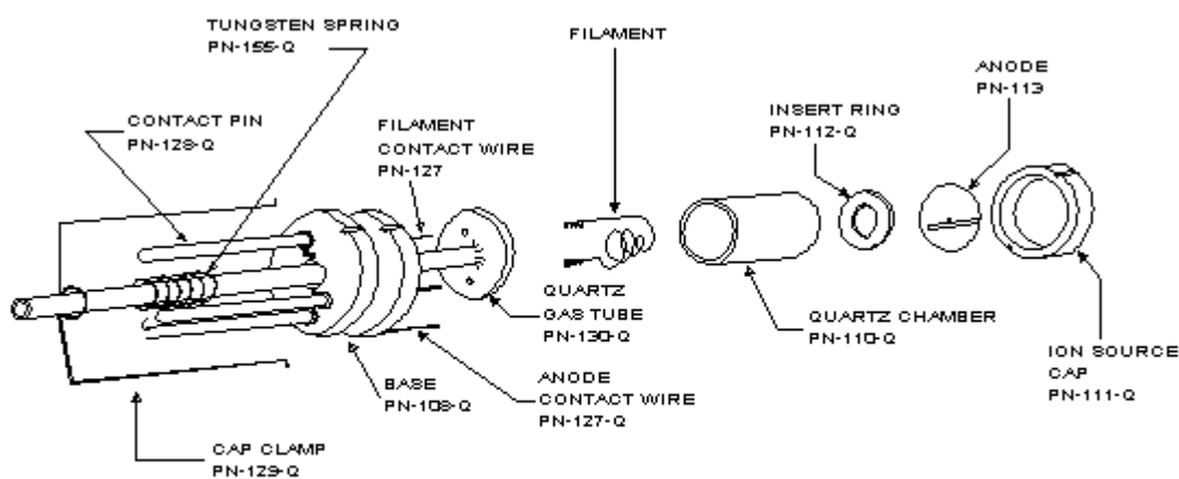
MODEL 101-Q ION SOURCE (Quartz)
