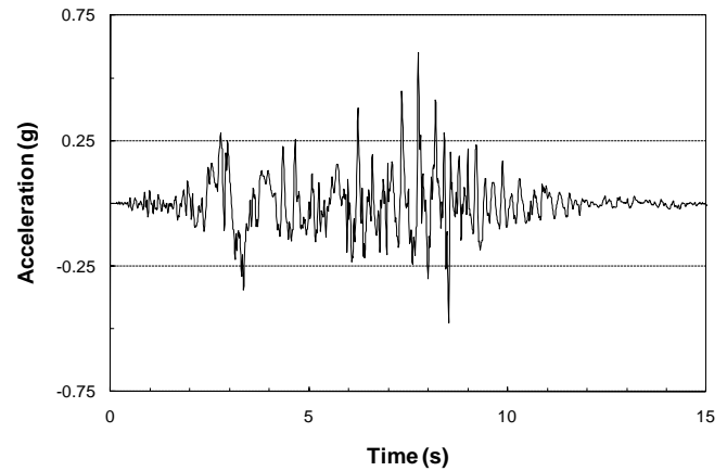
Fig. 3. Modified acceleration time history at the abutment of Pacoima Dam (Seed et al. 1973)
