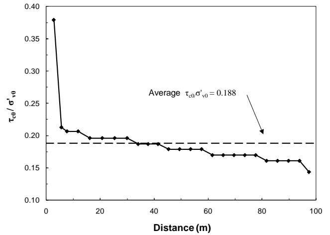
Fig. 7. \tau_{c0}/\sigma'_{v0} versus distance on the failure plane from the upstream shell.
