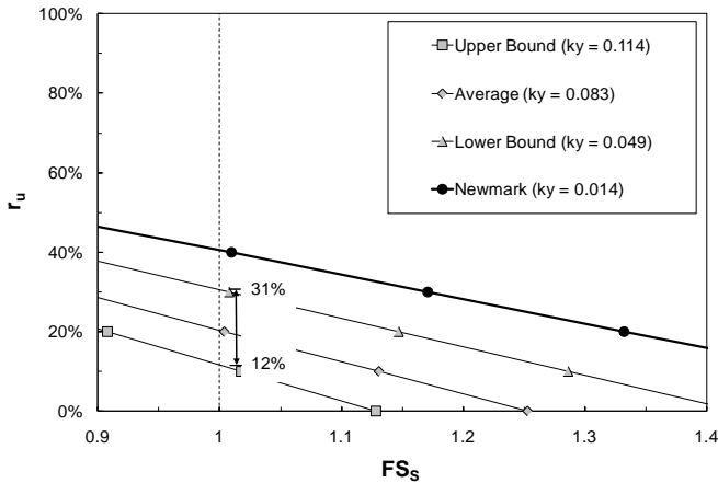
Fig. 9. FS_S for different r_u values in the core area corresponding to upper bound, average, and lower bound values of k_y from Makdisi-Seed's method and k_y from Newmark's analysis.
