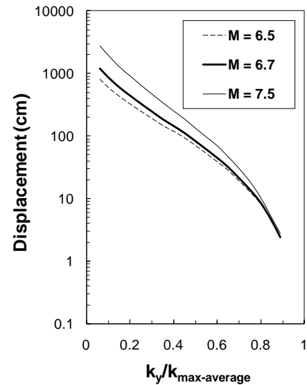
Fig. 5. Average values of the permanent displacement of an embankment caused by different levels of earthquake shaking (after Makdisi and Seed 1978).
