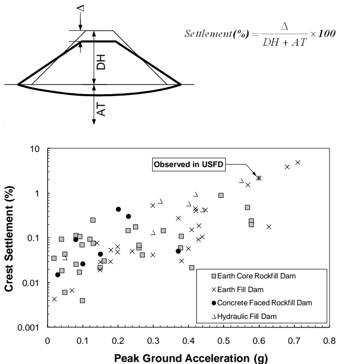
Fig. 6. Peak ground acceleration versus crest settlement (after Swaigood 2003)
