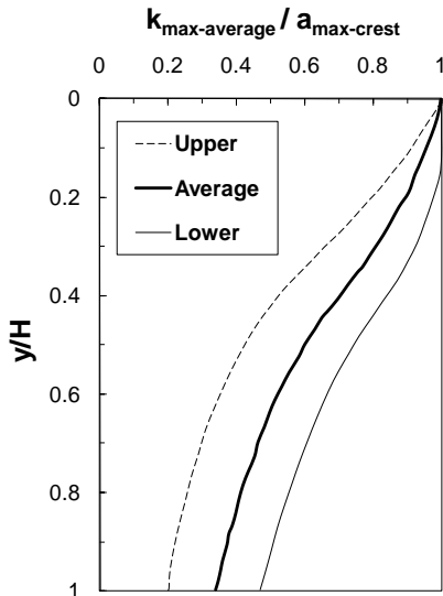
Fig. 4. Variation of the average peak acceleration coefficient ( k_{\max\text{-average}} ) with depth of the potential sliding mass ( y ) (after Makdisi and Seed 1978).
