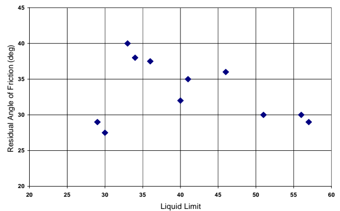
Fig. 4a. Liquid Limit vs Residual Angle of Friction
