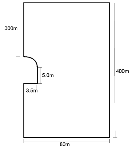
Fig.6. Dimensions and boundaries of the model for numerical analysis.
