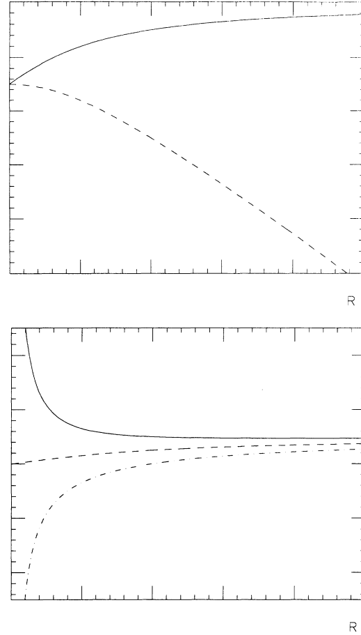
FIG. 1. (a) Plot of the functions \beta_1 (solid line) and \beta_0 (dashed line) when L = 0 . (b) Behavior of the effective potential V_+ when \beta > -|Q| (solid line), \beta = -|Q| (dashed line), and \beta < -|Q| (dot-dashed line).
