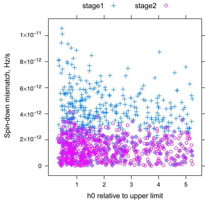
FIG. 5 (color online). Improvement of spin-down localization of injected test signals. The injected strain divided by the upper limit in this band (before injection) is shown on the x axis. The difference between injection spin-down and spin-down of corresponding outlier is shown on the y axis. Crosses, semicoherent; circles, loosely coherent.
