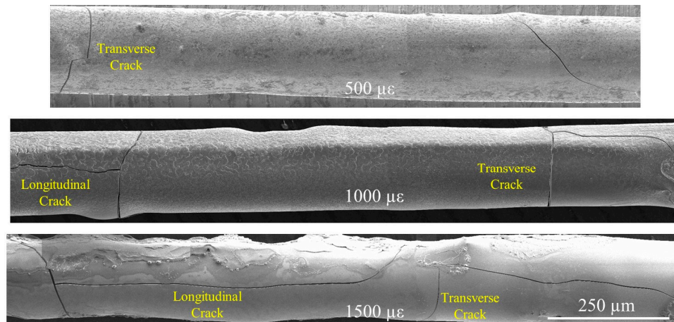
Figure 6. Stacked SEM images along axial direction of the fiber showing two adjacent transverse cracks at each strain.
