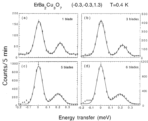
FIG. 1. Neutron scattering intensity with (a) one blade, (b) three blades, (c) five blades, and (d) six blades of the horizontally focusing analyzer, as a function of energy transfer at 0.4 K. These data were collected at (-0.3, -0.3, 1.3) with a final energy of 2.6 meV. Solid curves are Gaussian fits to the data.
