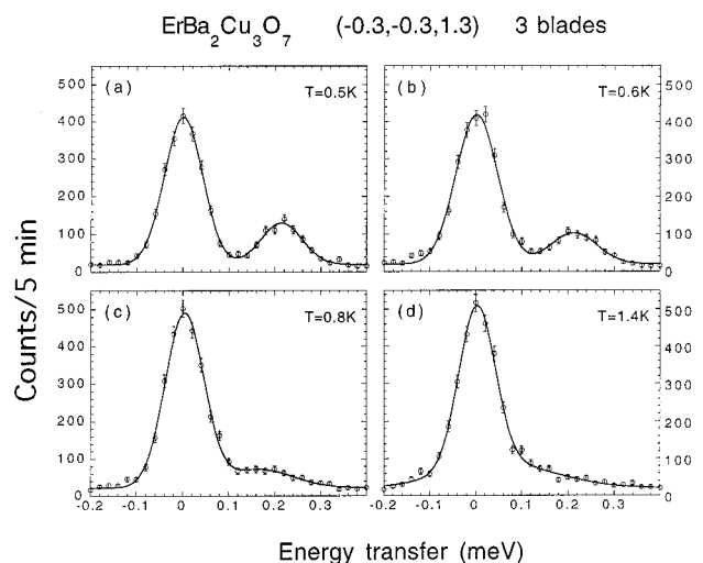
FIG. 3. The neutron scattering intensity as a function of energy transfer at (a) 0.5, (b) 0.6, (c) 0.8, and (d) 1.0 K. Solid curves are fits to the data.
