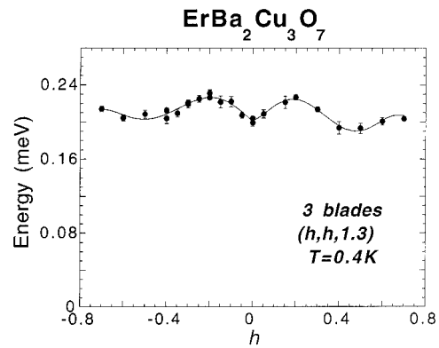
FIG. 2. The dispersion of magnetic excitations along (1,1,0) direction. The solid curve is a guide to the eye. There is a large gap in the excitation spectrum of about 0.2 meV, but with significant dispersion.
