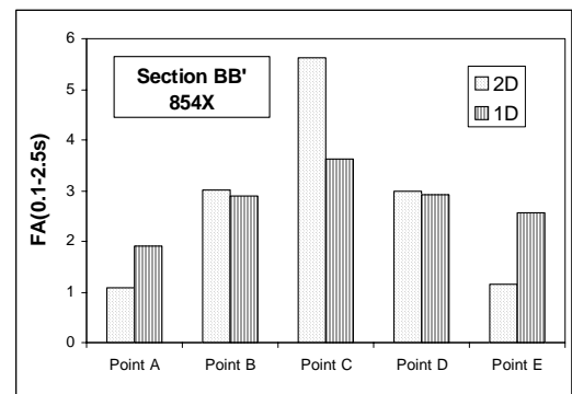
Fig. 11a. Amplification factors corresponding to 6 surficial points on section BB' for 854X input motion.
