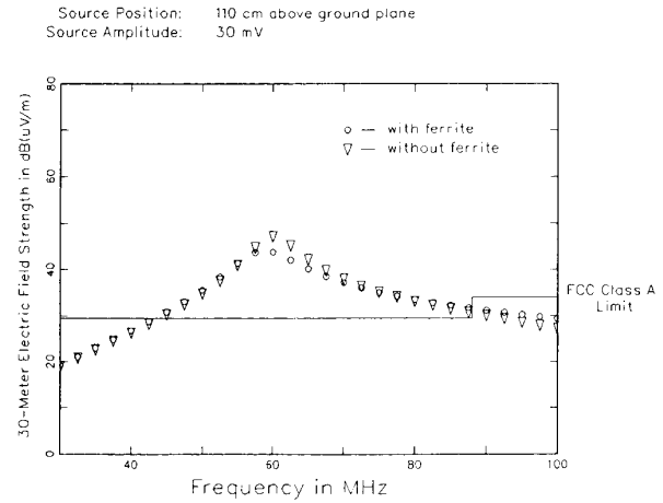
Fig. 14. Ferrite's effect on the radiation from the 120-cm wire.
