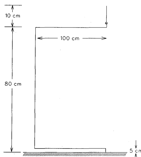
Fig. 8. End-driven wire model of test circuit with dc power supply.
