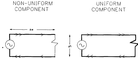
Fig. 22. Components of current distribution in a small circuit.
