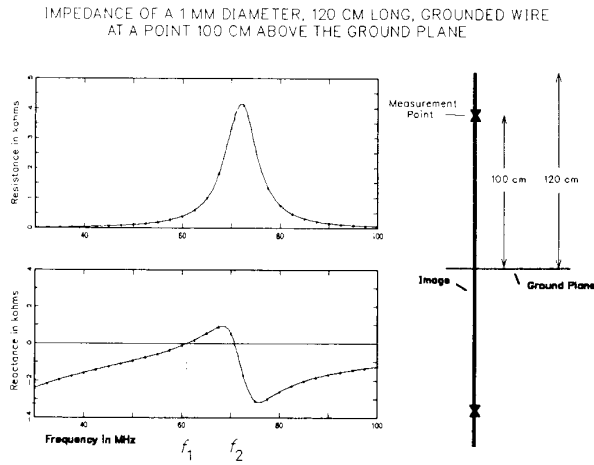
Fig. 12. Resistance and reactance near one end of a long wire.
