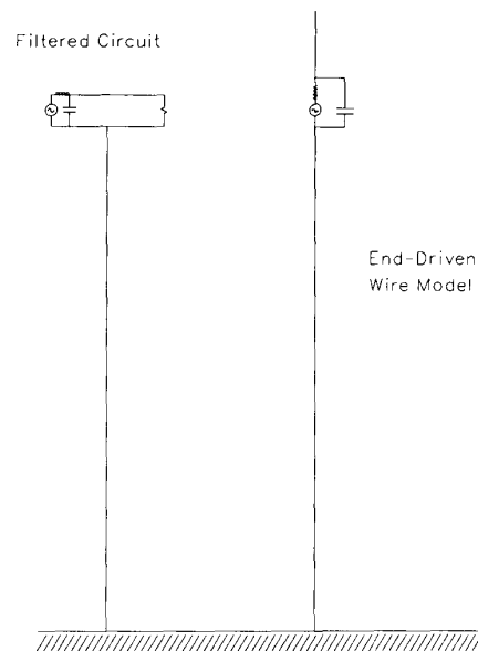
Fig. 11. End-driven wire model of a filtered circuit.
