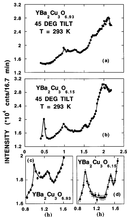
FIG. 3. (a) A scan along the 45^\circ direction for the 6.93 sample while (b) shows the same scan for the 6.15 antiferromagnet. The scale shown is the distance along the 45^\circ direction projected on the \mathbf{b}^* direction. (c), (d) Expanded versions of (a) and (b).
