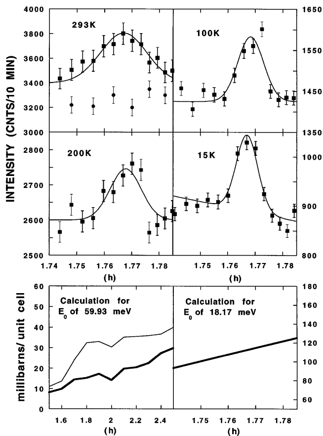
FIG. 4. The top four graphs show measured results obtained with an E_0 of 18.17 meV taken along the 7^\circ direction. The scale shown is the distance along the 7^\circ scan projected on the \mathbf{h}^* axis. Several scans were averaged to obtain the errors shown. The lines are least squares fits to a Gaussian distribution on a sloping background. The round points on the 293 K plot are measurements along an 18^\circ trajectory (see Fig. 1) for which the peak moves out of the scan range and thus serves as a measure of the background scattering. The lower graphs are the model simulations of the scans using a shell model.
