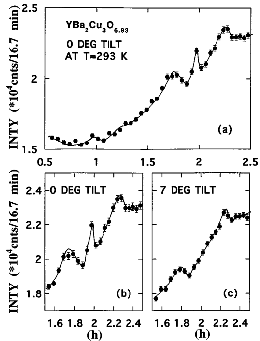
FIG. 2. (a) The result of a scan along \mathbf{b}^* or along the 0^\circ line. (b) An expanded version of the scan while (c) is the result obtained along the 7^\circ direction [see Fig. 1(b)]. Superlattice or satellite peaks are found around the Bragg peak positions for the larger Q reflections. Solid lines are guides to the eye.
