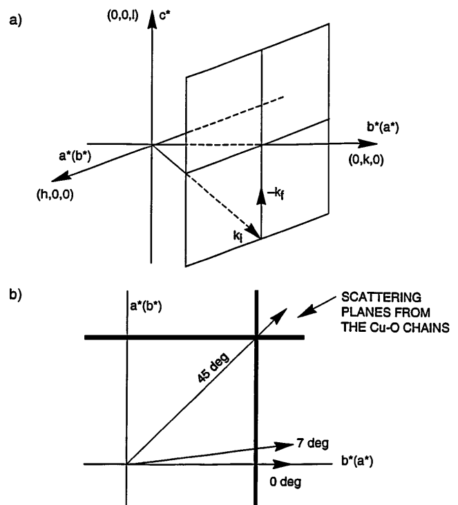
FIG. 1. (a) The scattering diagram used to achieve integration in planes perpendicular to \mathbf{b}^* . (b) The scan directions used in the measurements. Two sets of planes result from the twinned crystal. These planes cross on the 45° scan which is in the [1, 1, 0] direction.
