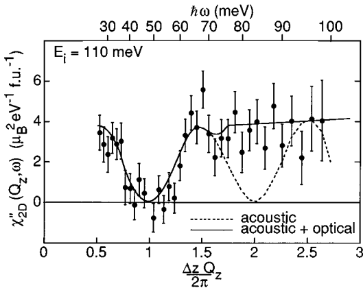
FIG. 3. Data collected with E_i = 110 meV, integrated over the spin-wave cones in the (Q_x, Q_y) plane near Q = (\frac{1}{2}, \frac{1}{2}, l) and corrected for the \text{Cu}^{2+} magnetic form factor and Bose factor. The resulting spectrum is collected along a trajectory in (Q_z, \hbar\omega) defined on the upper and lower axes. Under these conditions the sinusoidal intensity modulation with Q_z will disappear at \hbar\omega_g \approx 74 meV. Solid line corresponds to a fit to spin wave theory. Dotted line is the acoustic mode contribution.
