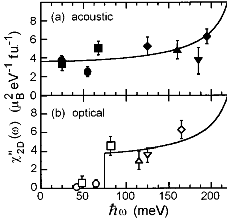
FIG. 2. The 2D local susceptibility as a function of energy transfer obtained by integrating over spin-wave peaks and correcting for the \text{Cu}^{2+} magnetic form factor, Bose factor, and instrumental resolution. (a) acoustic positions and (b) optical positions. The figure is a compilation based on the analysis of data such as those in Fig. 1 with various incident energies. Solid lines correspond to fits to spin wave theory.
