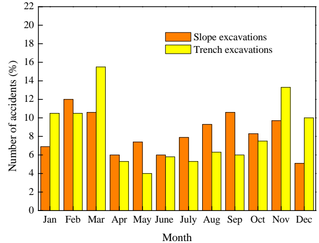
Fig. 15. Number of slope and trench failures by month.
