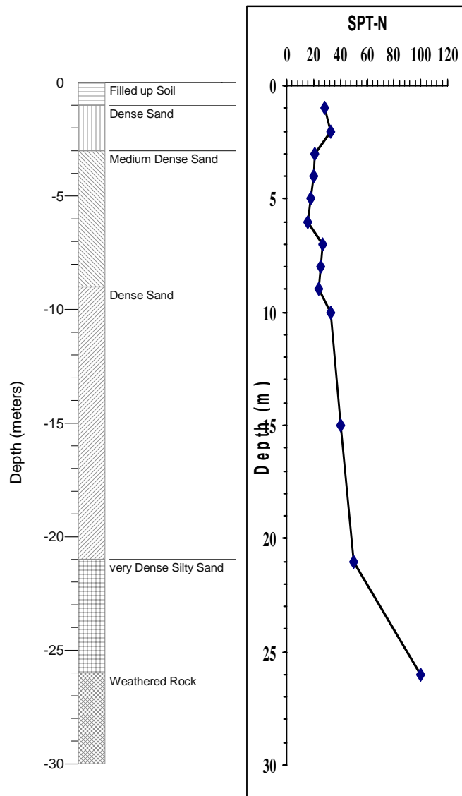
Fig. 2. Borelog and variation of SPT-N with depth
