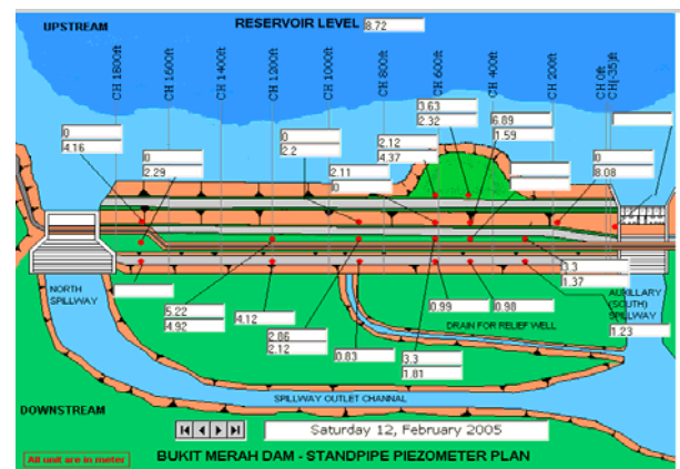
Fig. 5. Location of the piezometers for Bukit Merah Dam
