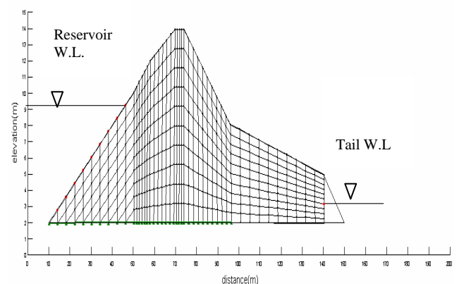
Fig. 8. Discretization of the domain of Bukit Merah Dam cross-section into finite elements meshes
