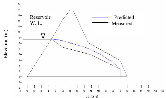
Fig. 13. Observed and predicted phreatic surfaces for Bukit Merah Dam at CH 180 m (Maximum water level in the reservoir)
