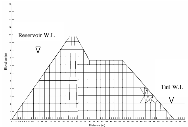
Fig. 7. Discretization of the domain of Labong Dam cross-section into finite elements meshes
