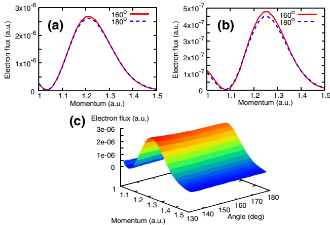
FIG. 3 (color online). Electron wave packets extracted from photoelectron momentum images along the BRR are shown to be identical for scattering angles of 160^\circ and 180^\circ , extracted from (a) H target, (b) Ar target, using the same ionizing laser. (c) The extracted electron wave packet from H target is the same over the angular range of 130^\circ to 180^\circ .
