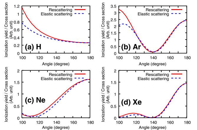
FIG. 2 (color online). Angular distributions of photoelectrons along the BRR compared to the differential elastic scattering cross sections of the target ion. Each BRR is taken to be the outer half circle on the right side of Figs. 1(c) and 1(d), respectively. (a) for H target, (b) for Ar, (c) for Ne, (d) for Xe.
