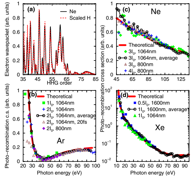
FIG. 4 (color online). (a) Comparison of the “electron wave packets” extracted from the HHG spectra of Ne and scaled H generated by a 5.2 fs laser pulse with peak intensity of 2 \times 10^{14} W/cm ^2 and mean wavelength of 1064 nm. Extracted photo-recombination cross sections from the HHG, of Ar (b), Ne (c) and Xe (d), using different laser pulses, plotted vs the photon energy. For each panel, the dashed red line denotes the calculated photo-recombination cross sections by free electrons. ( I_0 = 10^{14} W/cm ^2 .)
