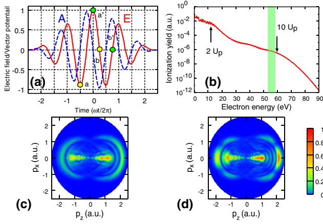
FIG. 1 (color online). (a) Schematic of the electric field ( E ) and the vector potential ( A ) of a typical few-cycle pulse. (b) Electron energy spectra of atomic hydrogen ionized by a 5 fs (FWHM) laser pulse, with mean wavelength of 800 nm and peak intensity at 10^{14} W/cm ^2 . (c) Normalized 2D photoelectron momentum spectra of atomic hydrogen. The images are renormalized for each photoelectron energy to reveal the global angular distributions. (d) Momentum images of Ar in the same pulse.
