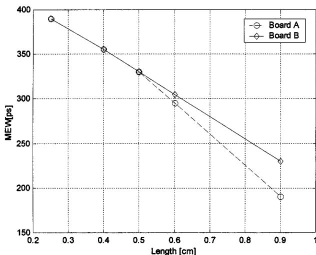
Fig. 11. Predicted MEW for different lengths of the stripline at 2.5 Gb/s.
