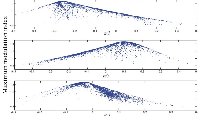
Figure 7. Coefficient selection for maximum modulation index.
