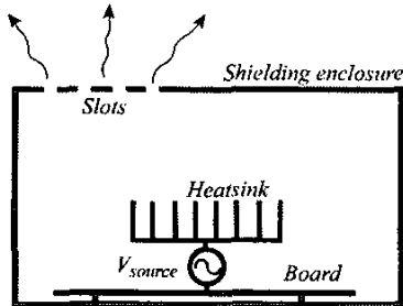
Fig. 4. Radiation due to a heatsink driving enclosure resonances within a shielding enclosure
