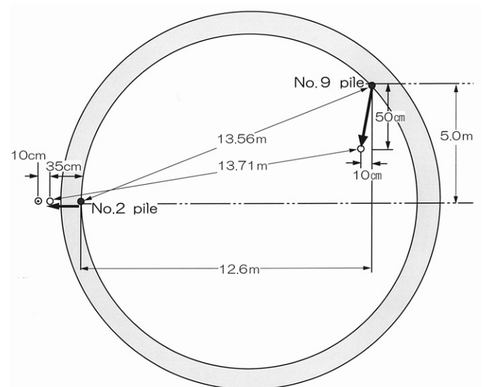
Fig. 13. Permanent lateral displacements of Pile No. 2 and Pile No. 9 at the head of the pile
