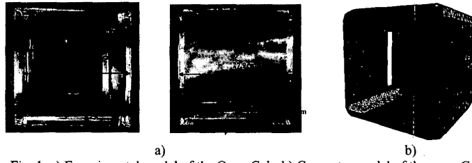
Fig. 1. a) Experimental model of the Open Cub; b) Computer model of the open Cub
