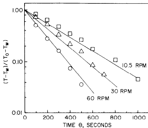
FIG. 1. Experimental temperature approach for Cabosil (2.3 wt%).
