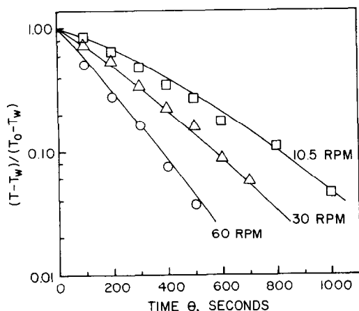
FIG. 2. Experimental temperature approach for Cabosil (2.3 wt%).
