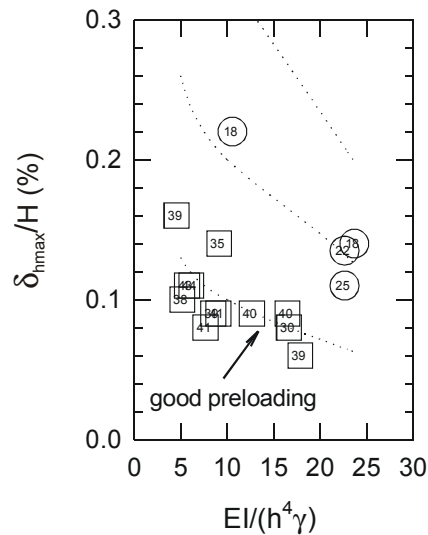
Figure 12. Effectiveness of pre-loading in control of lateral displacements. Numbers indicate measured pre-load expressed as a percentage of design load.
