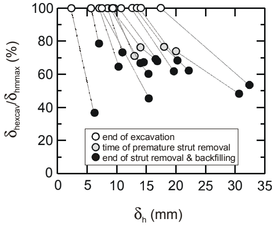
Figure 6. Proportion of maximum lateral displacement, \delta_{\text{hmax}} , occurring during various construction stages.
