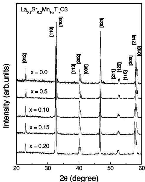
FIG. 1. X-ray diffraction patterns of \text{La}_{0.7}\text{Sr}_{0.3}\text{Mn}_{1-x}\text{Ti}_x\text{O}_3 ( 0 \leq x \leq 0.20 ) at room temperature.
