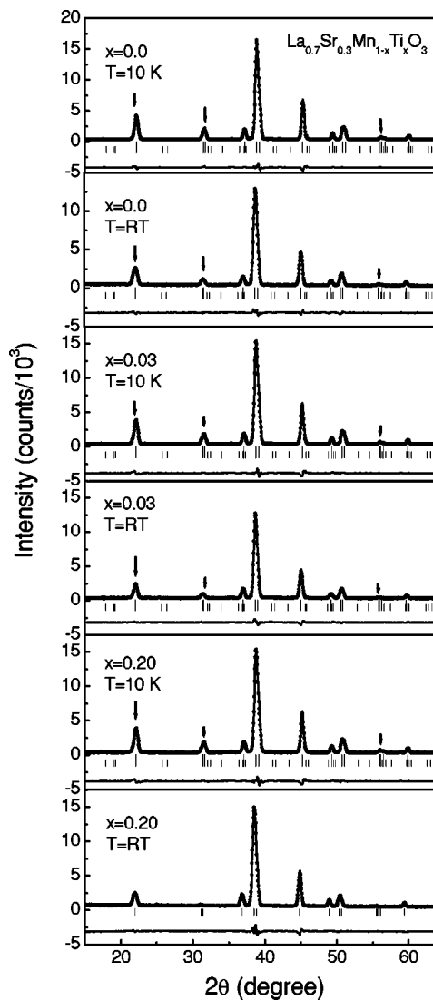
FIG. 2. Neutron-diffraction patterns of \text{La}_{0.7}\text{Sr}_{0.3}\text{Mn}_{1-x}\text{Ti}_x\text{O}_3 ( x=0.0, 0.03, \text{ and } 0.20 ) at 10 K and RT. [The bottom curves ( Y_{\text{obs}}-Y_{\text{cal}} ) are the difference between experimental data and refinement data. The vertical bars indicate the magnetic (bottom) and Bragg (top) peak positions.] Arrows indicate some of major magnetic diffraction peaks.
