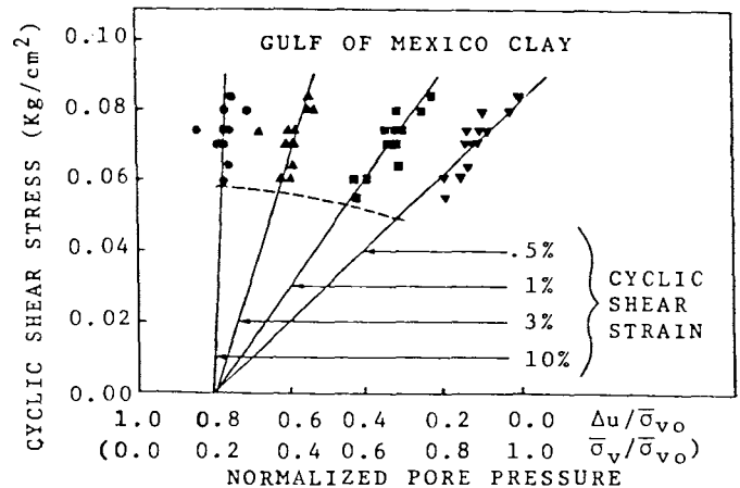
Fig. 6 Cyclic Shear Stress versus Normalized Pore Pressure
