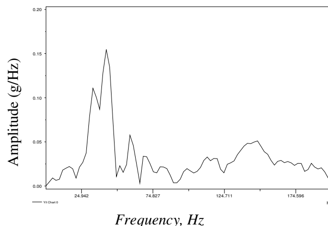
Fig.10. Typical Spectrum of horizontal ground acceleration at a distance of 3m from the centre of pile
