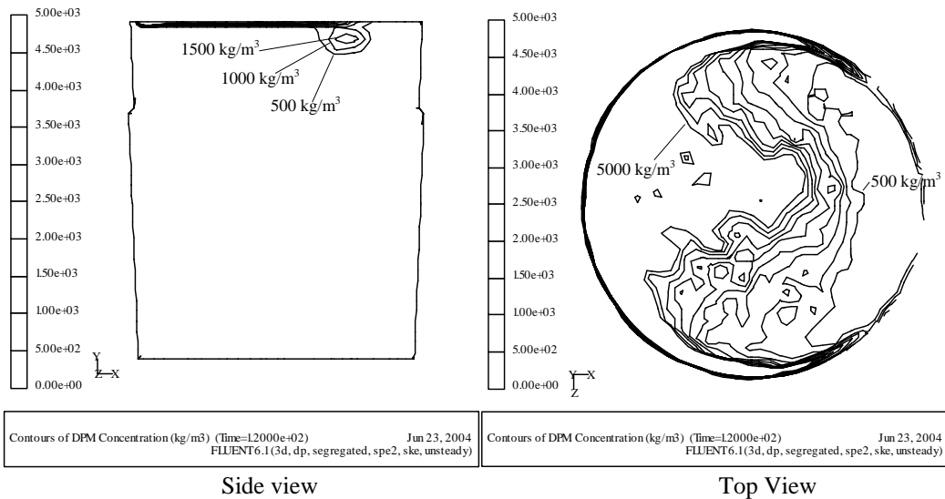
Figure 8 Ferroalloy particle distribution during addition (20 seconds after start of ferroalloy addition - FLUENT output)
