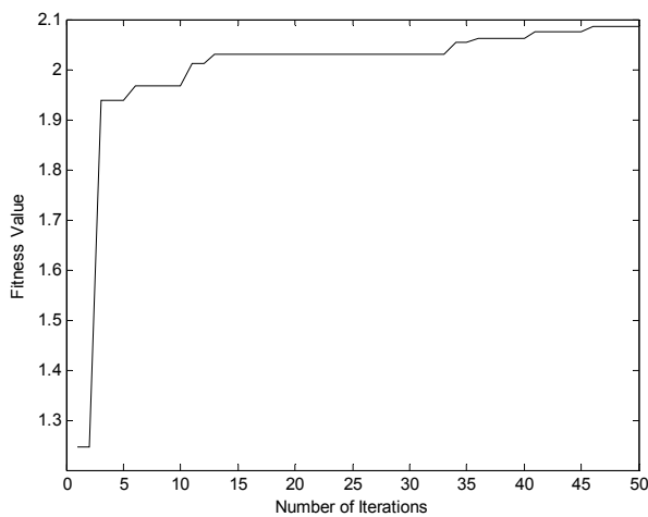
Fig. 6. Fitness of gbest particle over the entire simulation
