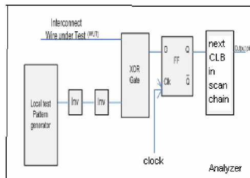
Fig 4 Block diagram of Analyzer
