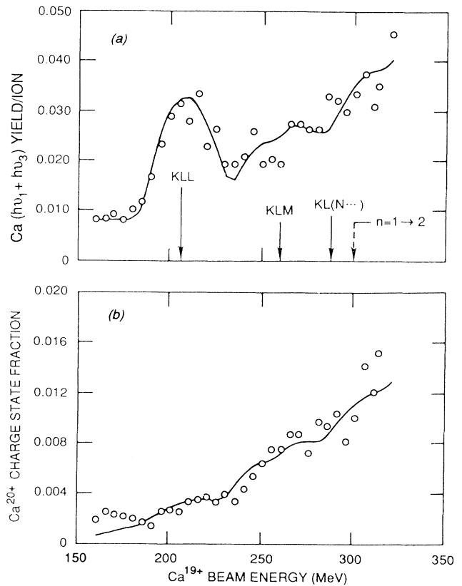
FIG. 1. (a) Yield of h\nu_1(2nl' \rightarrow 1snl) plus h\nu_3(2l \rightarrow 1s) calcium x rays [see Eq. (1)] and (b) charge fraction of Ca^{20+} ions as a function of Ca^{19+} ion energy incident on a \langle 110 \rangle channel in Si (1.2 \mu\text{m} thick). The smooth curves are results of a computer simulation as described in the text.
