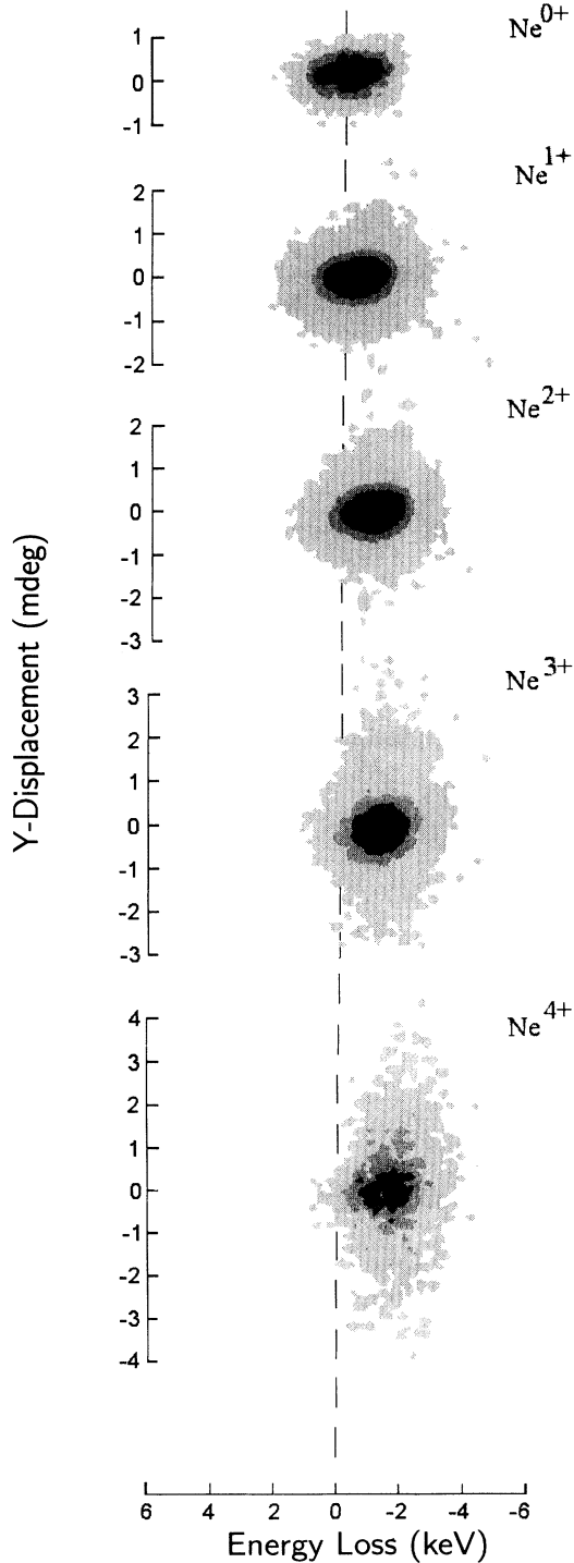
FIG. 4. Two-dimensional contour plot of projectile ion distributions in coincidence with recoil-ion charge state for direction ionization, i.e., C^{6+} + Ne \rightarrow C^{6+} + Ne^{q+} + qe^- . Ne^{0+} represents the projectile that did not ionize any target electrons.
