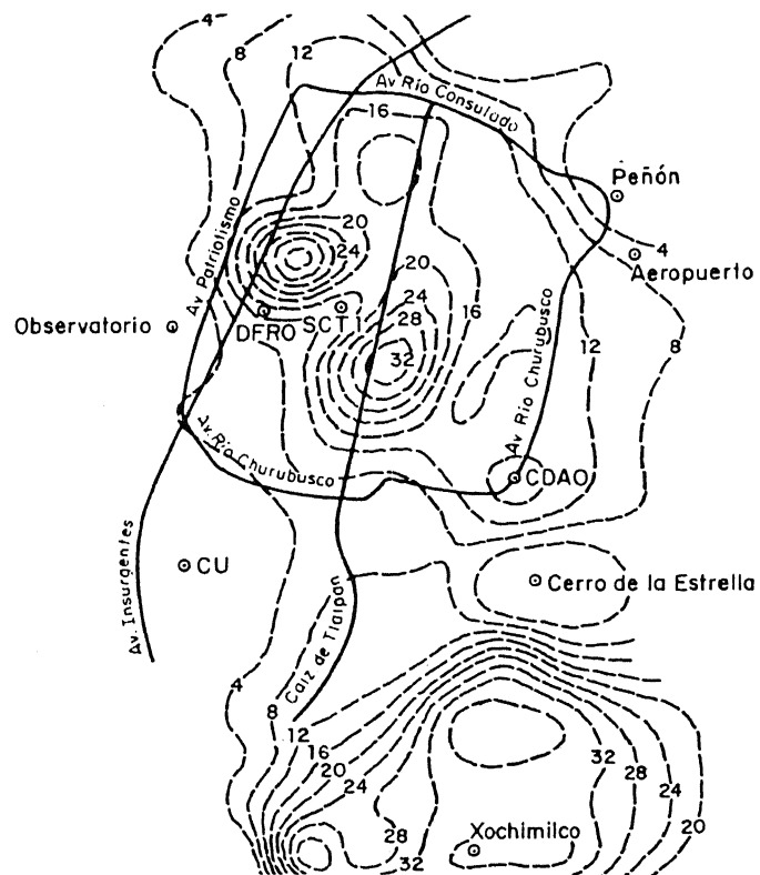
Fig 3 Maximum normalized energy contours, March 25, 1989
