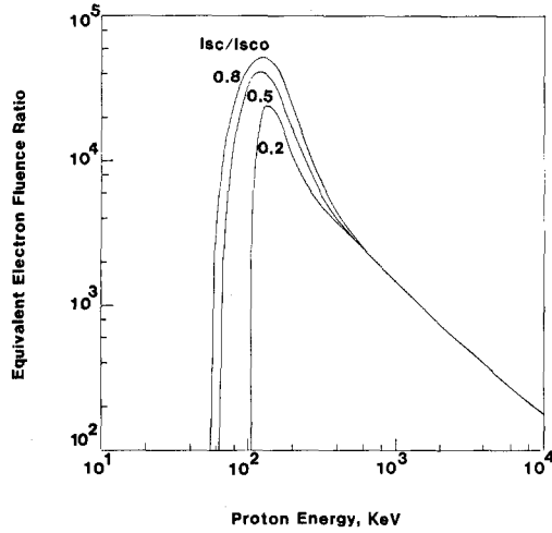
Fig. 3. Equivalent electron fluence ratio for GaAs heteroface solar cells with an 0.4- \mu\text{m} (GaAl)As window and 0.5- \mu\text{m} junction depth as a function of proton energy for three different damage levels.
