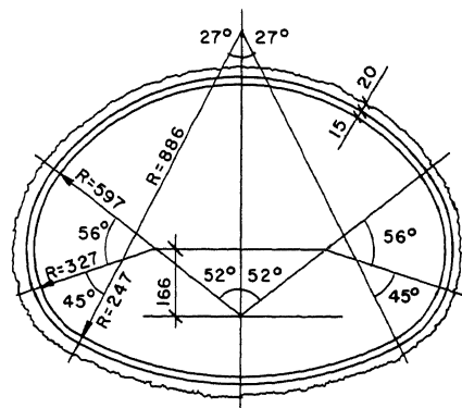
Fig. 2 Typical cross section of the Paraíso tunnel (dimensions in centimeters)
