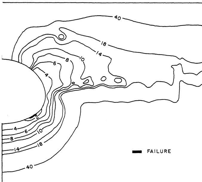
Fig. 11 Isostress-ratio curves
