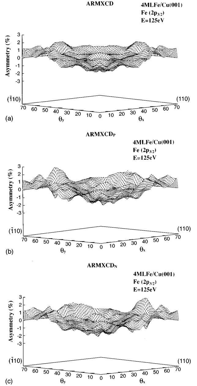
FIG. 7. Spin-summed angle-resolved magnetic circular dichroism as a function of (\theta, \phi) in a quadrant bounded by the (110) and (\bar{1}10) azimuths, (a) for \text{ARMXCD} , (b) for \text{ARMXCD}_P , and (c) for \text{ARMXCD}_N .
