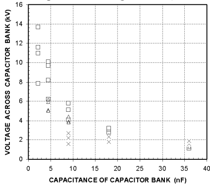
Figure 3. Amplitude of the voltage pulse produced by FEGs containing \text{Pb}(\text{Zr}_{52}\text{Ti}_{48})\text{O}_3 disk with D = 27 \text{ mm}/h = 0.65 \text{ mm} (crosses), D = 25 \text{ mm}/h = 2.1 \text{ mm} (triangles) and D = 25 \text{ mm}/h = 5.1 \text{ mm} (squares) across capacitor banks of different capacitance.
