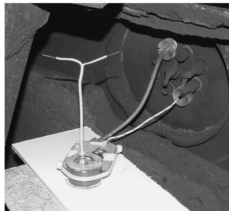
Fig. 2. High-voltage FMG prepared for explosive and electrical operation. The generators contained Nd_2Fe_{14}B energy-carrying element with an outer diameter of 25.4 mm, inner diameter of 8 mm, length of 19 mm, and pulse-generating coil of 252 turns.
